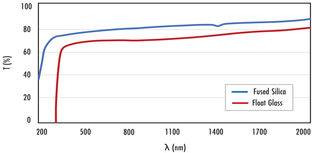
Ground Glass Diffusers Typical Transmission
