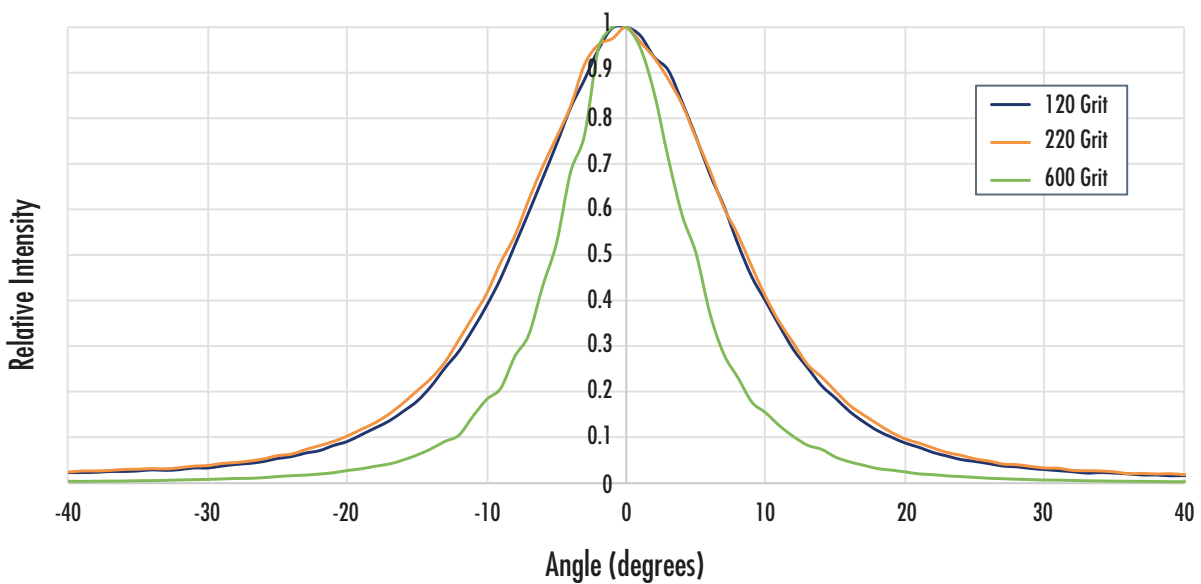
Relative Intensity vs. Angle for 120, 220 and 600 Grit
