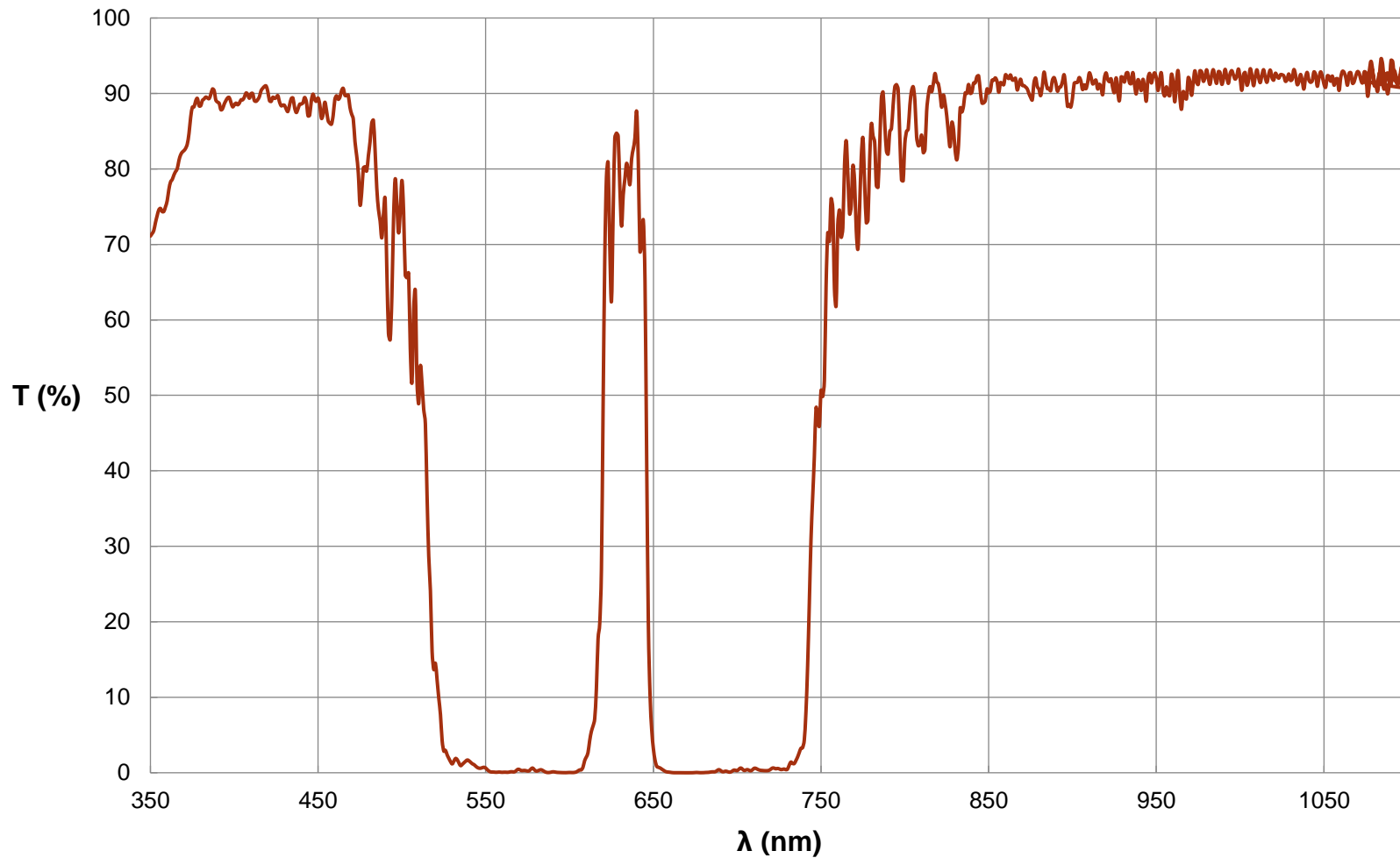
Everix Ultra-Thin Bandpass Filter, 630nm, OD 2.0 FOR REFERENCE ONLY
