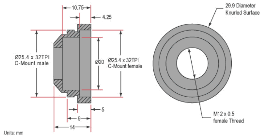
C-Mount Adapter (#53-675)
