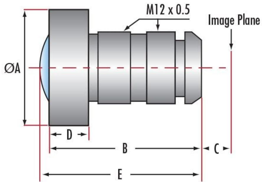
Infinite Conjugate M12 Imaging Lenses
