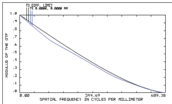
Typical Performance, #47-443 GRADIUM® Lens (Monochromatic Illumination)
