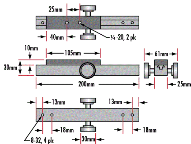
#53-384 Long Travel Single Axis
