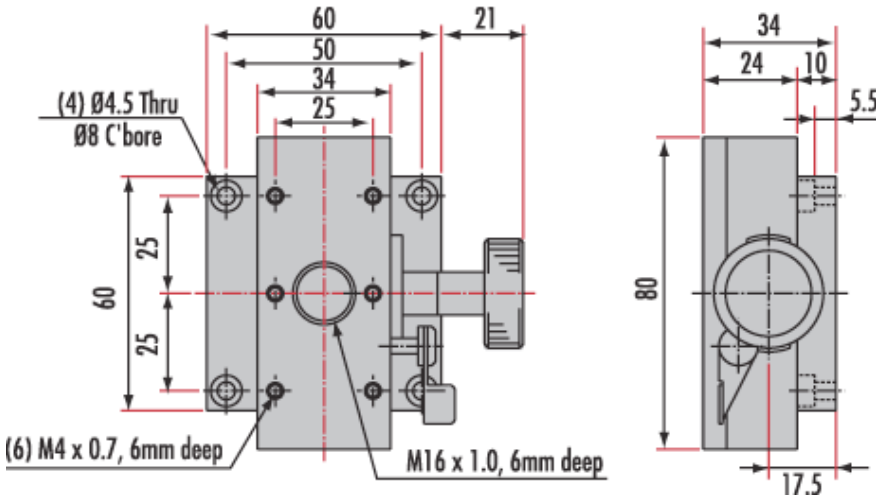
#55-026 - 60mm Travel, X-Axis Rack & Pinion Stage
